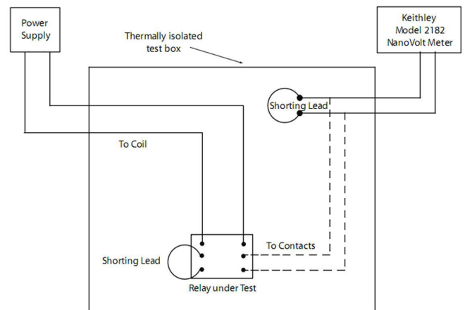
Figure 10. Double pole relay thermal offset voltage measurement setup.
