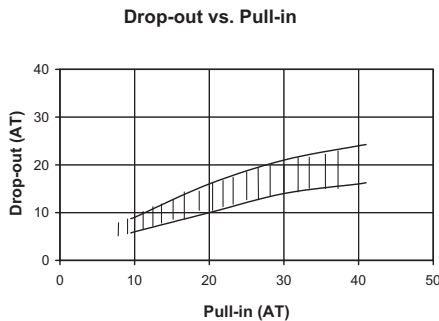
Fig. #7 The Pull-in and Drop-out ranges are shown. Note that variation in hysteresis for low ampere turns (AT) is very small and increases with higher AT.
