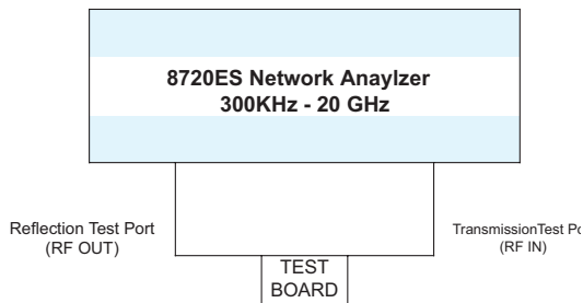
Fig. #14 Test Setup.
