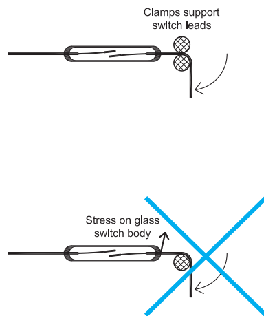
Fig. #1 Presentation of the proper and improper way of bending a Reed Switch. Supporting the switch lead while bending is a must.
