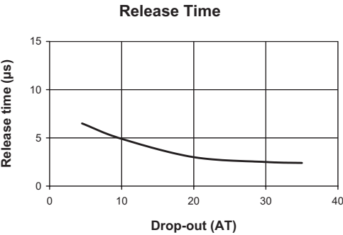
Fig. #16 A graph of the release time for increasing Dropout AT. With increasing Drop-out AT the restoring force increases causing even faster release time.
