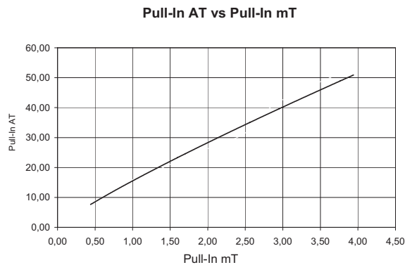
Fig. #9 The Pull-In AT is presented with its corresponding mT Pull-In level .
