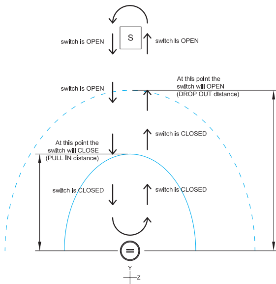
Fig. #29 Motion of the magnet is depicted in the y-z axis where the magnet is parallel to the Reed Switch, but moving perpendicular to its plane. The closure, holding, and opening points are shown.
