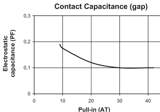
Fig. #18 As the Pull-in AT increases its gap increases, therefore reducing the capacitance across the Reed Switch.
