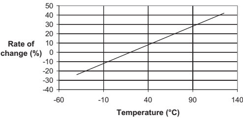
Fig. #6 The Pull-In and Drop-Out points will change with temperature at the rate of 0.4% /°C.
