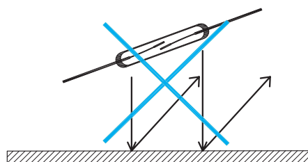
Fig. #5 Dropping the Reed Switch on a hard surface can induce several 100 G to the contacts many times altering the switch characteristics.
