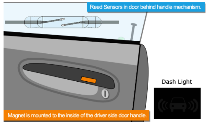
Figure 2. Illustration shows reed sensor in its normally open state. Car lock is unlocked and alarm not activated.
