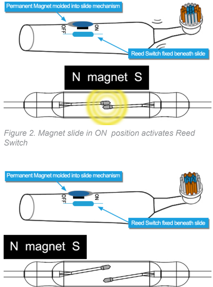
Figure 3. Magnet slide in OFF position deactivates Reed Switch
