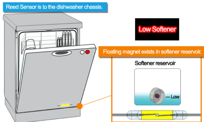
Figure 3. When the water softener fluid reaches a low level, the floating magnet will activate the reed switch sensor which is mounted outside the reservoir and at the base of the dishwasher.
