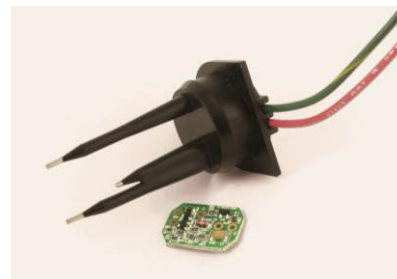
Conductive liquid level sensor
